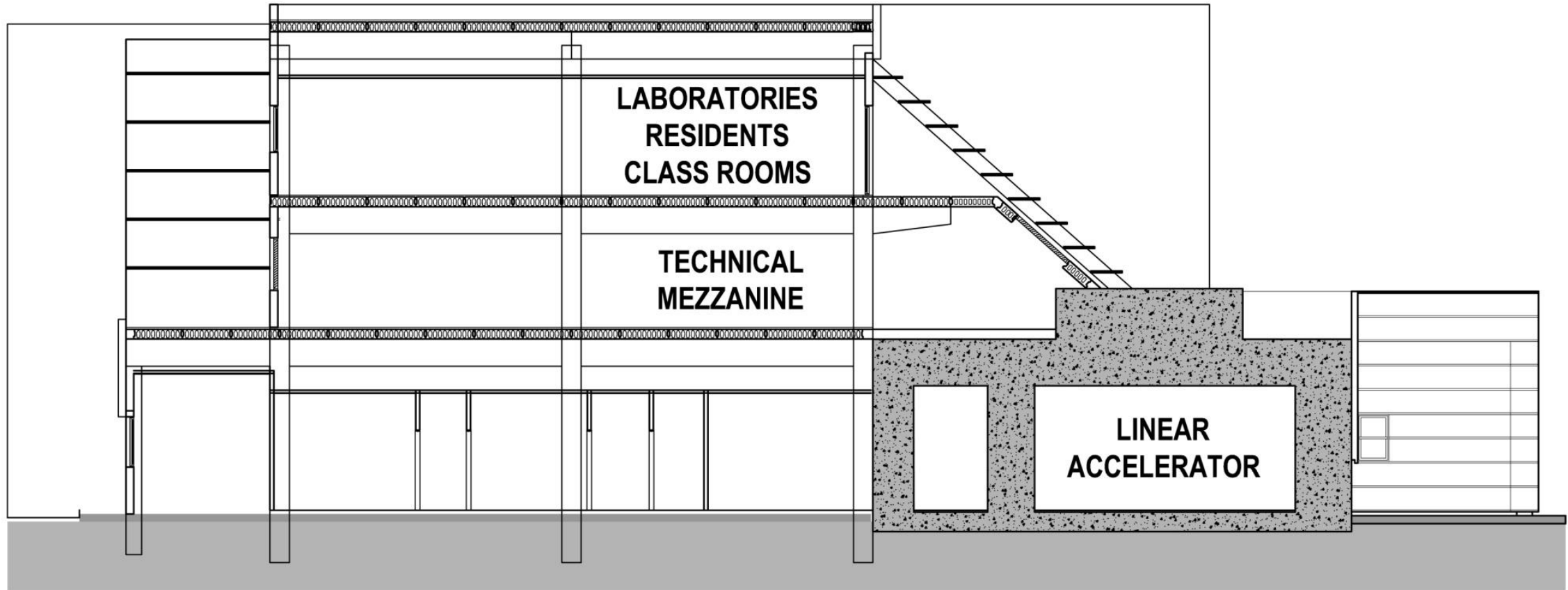
TECHNICAL SECTION B-B'
